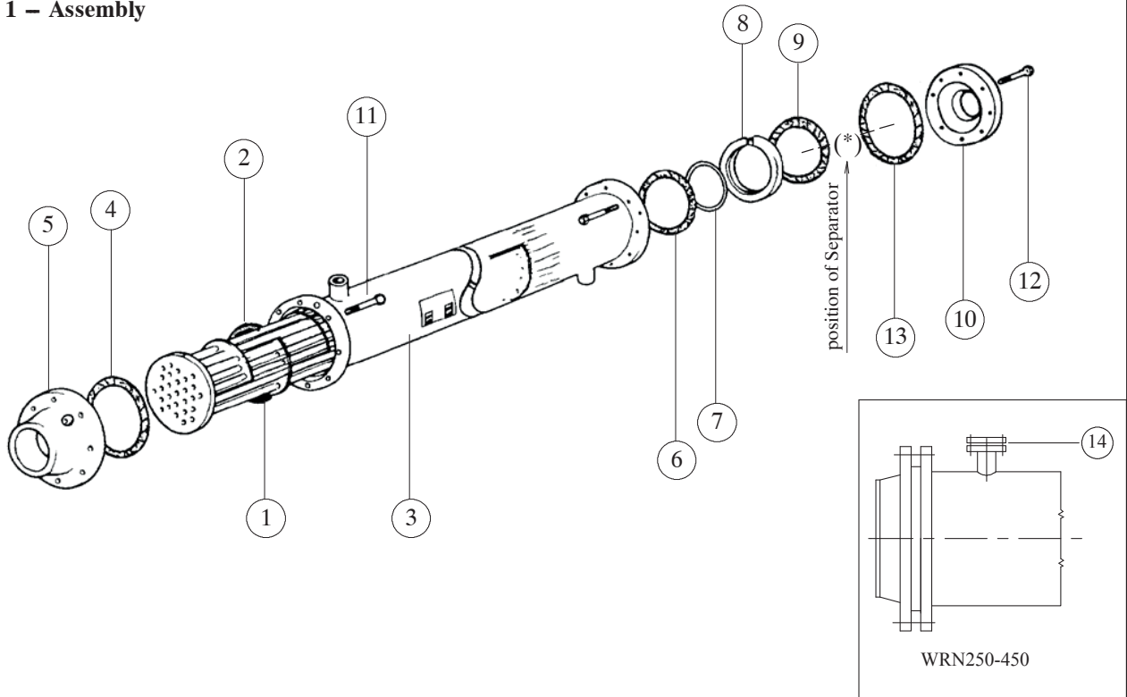
Fig. 1 – Assembly
